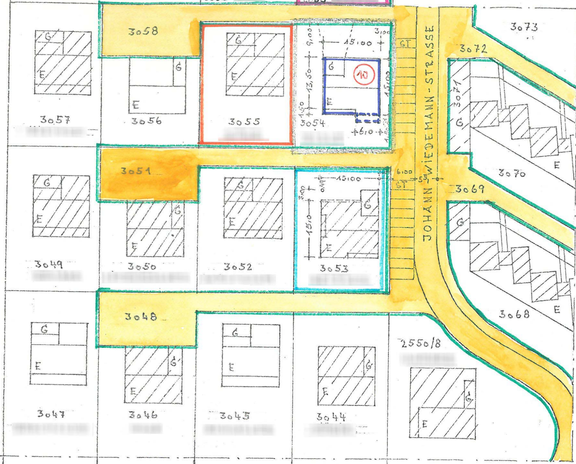
LAGEPLAN MS = 1:1000
